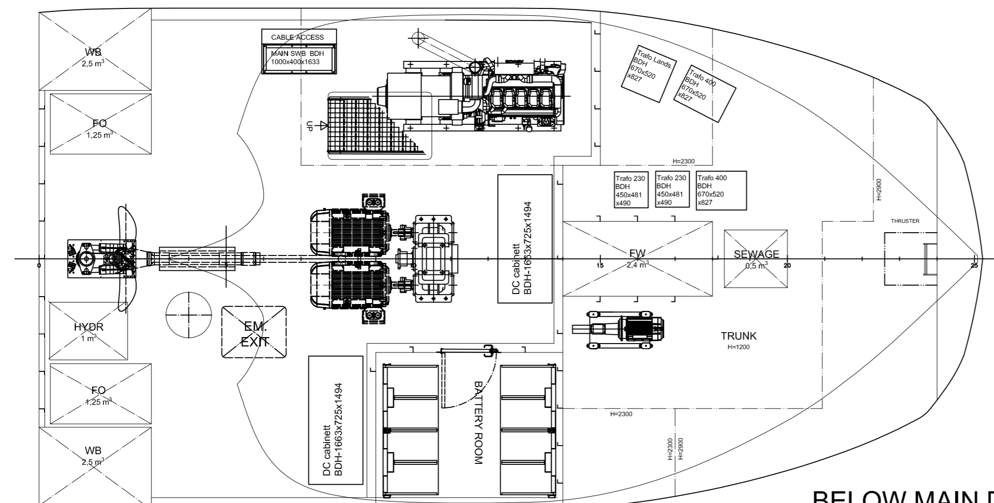
BELOW MAIN DECK 900
