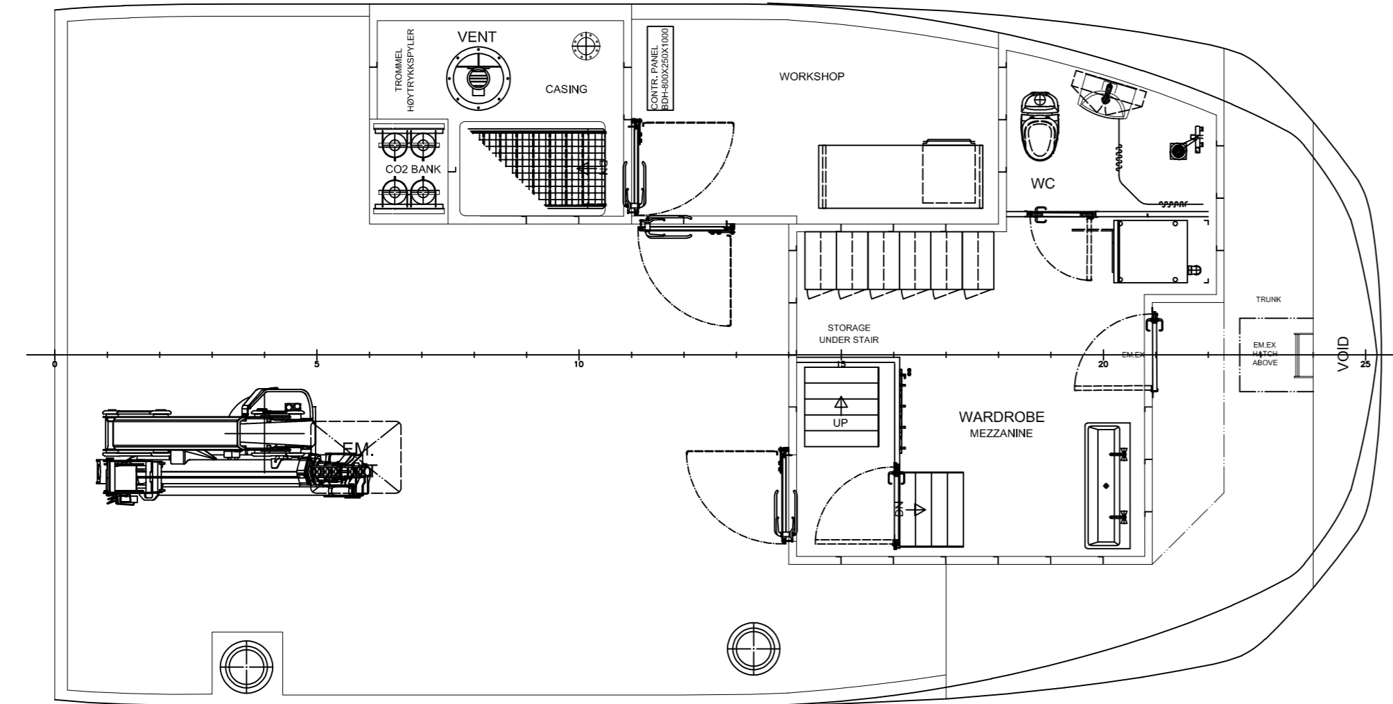
MAIN DECK 3200
