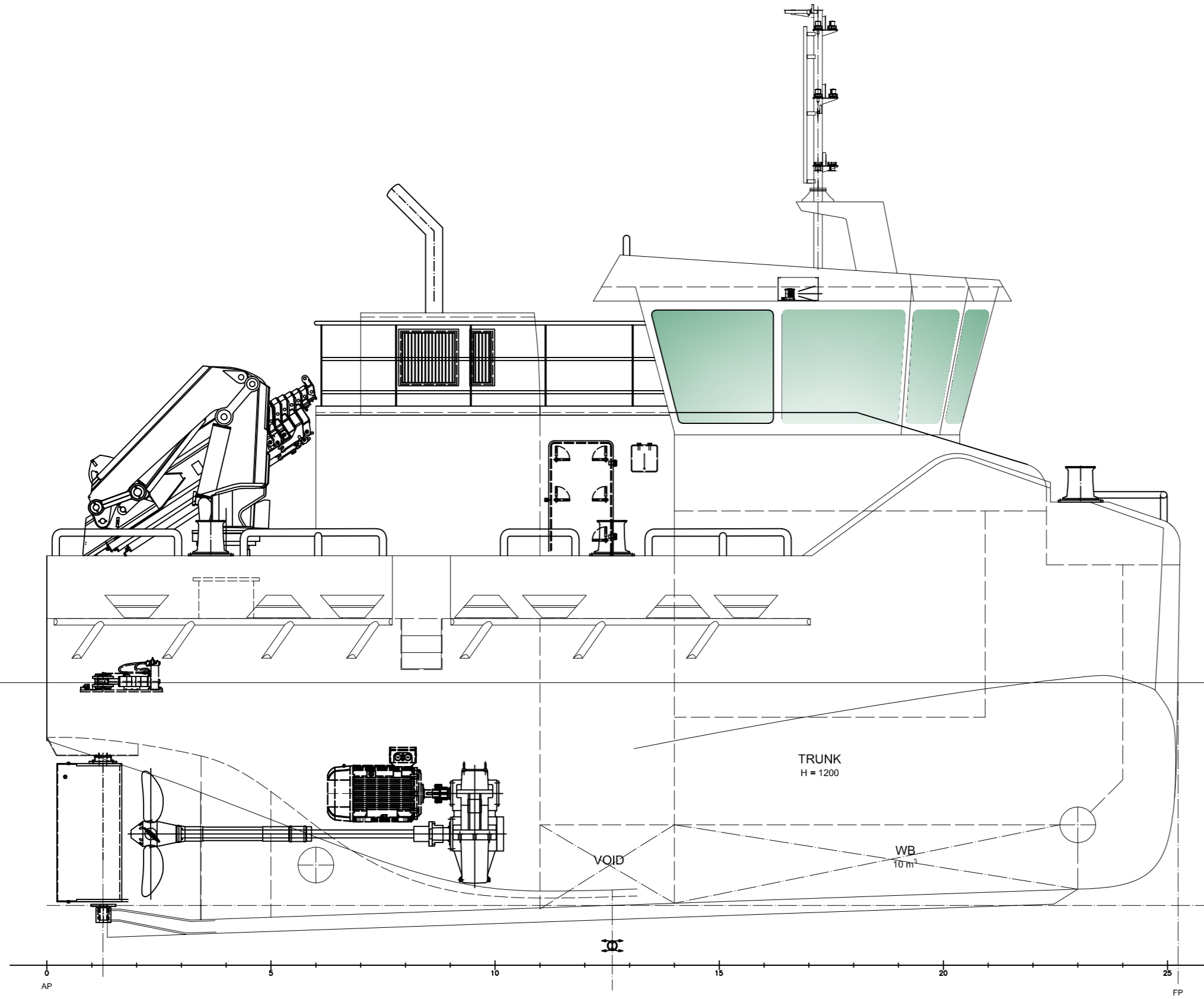
SB PROFILE
