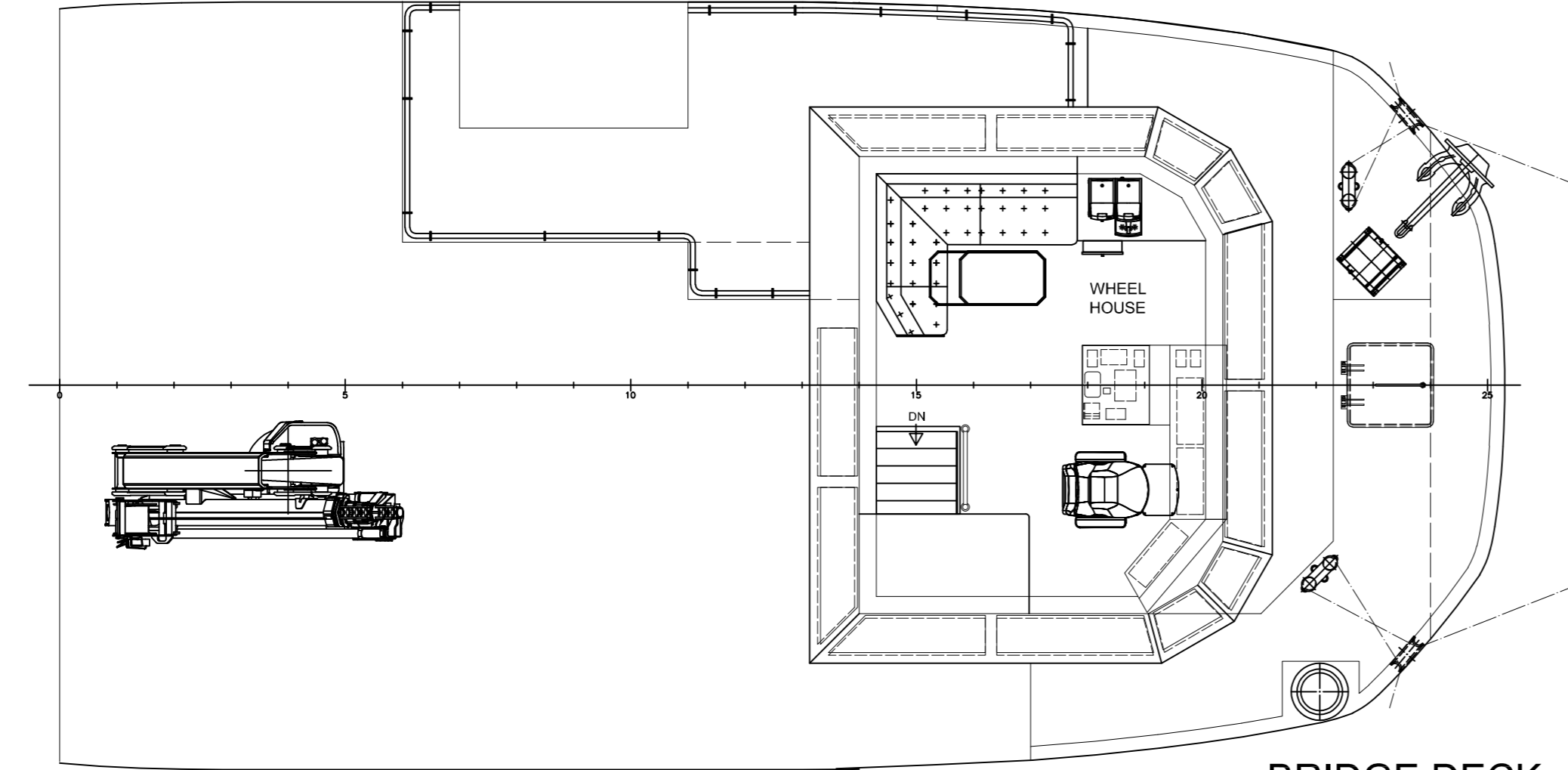
BRIDGE DECK 5500
