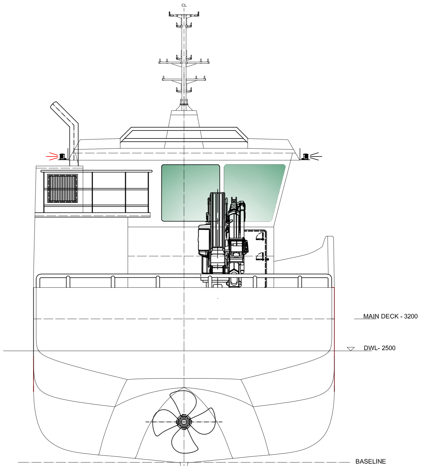
STERN VIEW
