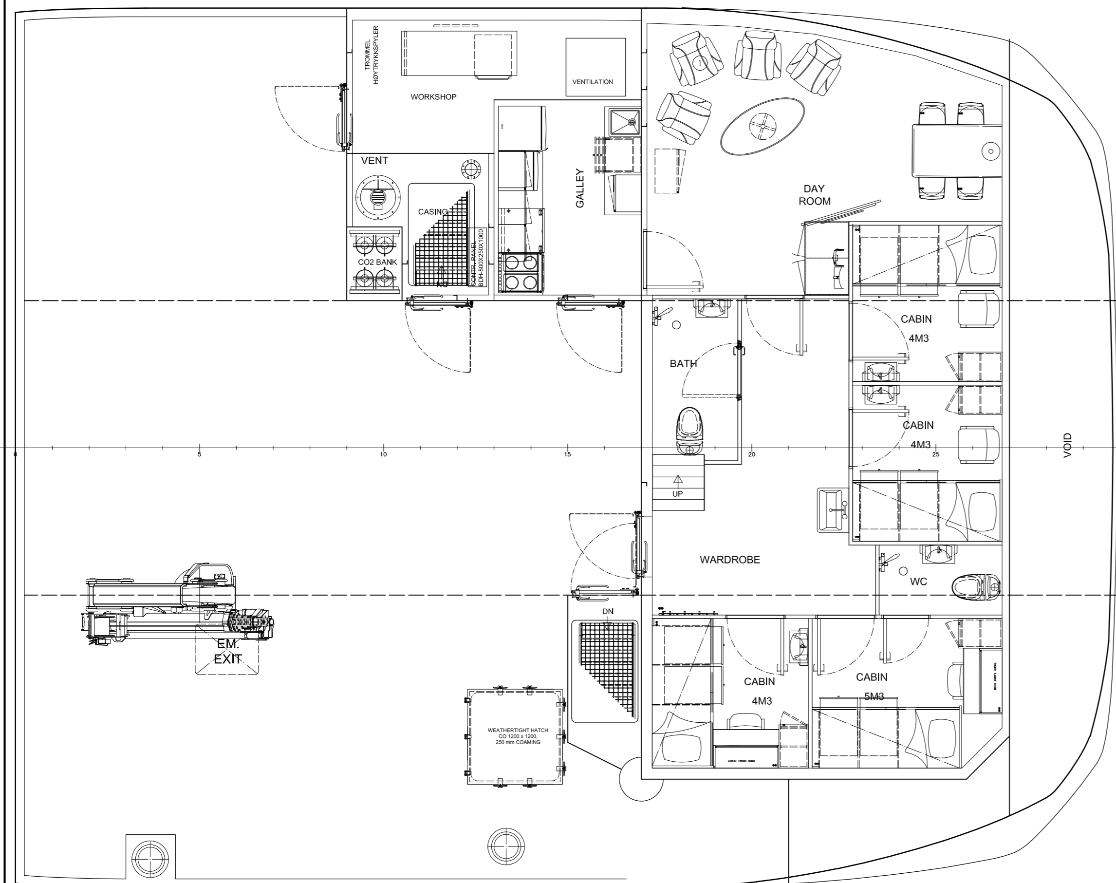
MAIN DECK 4000
