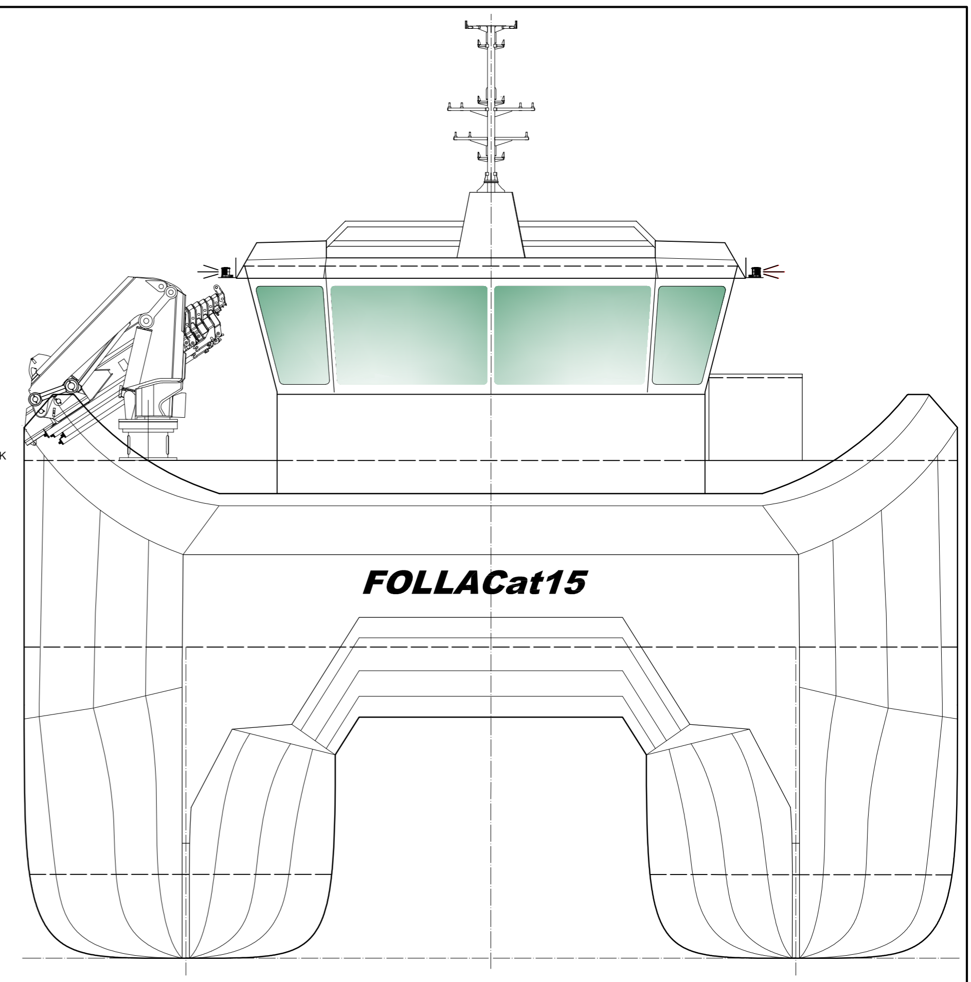
FRONT VIEW
