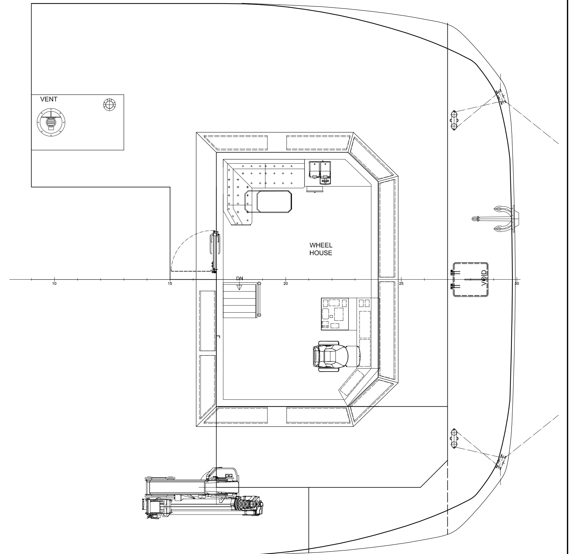
BRIDGE DECK 6400
